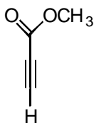
methyl propynoate
