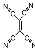
tetracyanoethylene
