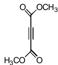
dimethyl acetylenedicarboxylate
