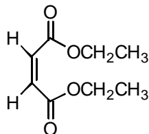
diethyl maleate
