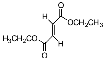
diethyl fumarate
