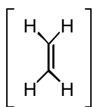
ethylene (unreactive)
